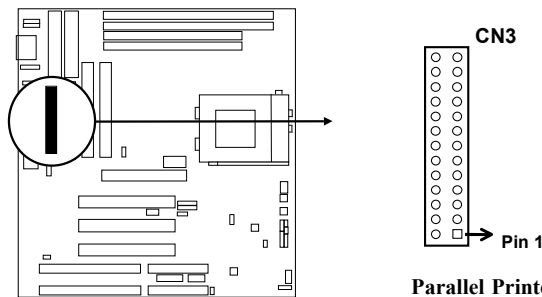
Parallel Printer Connector
