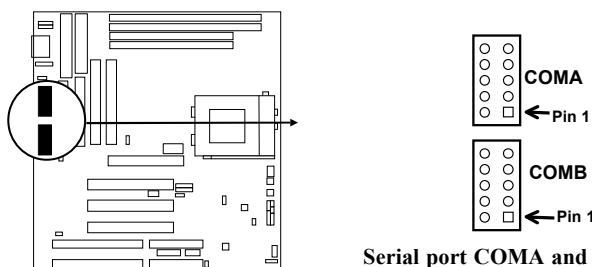
Serial port COMA and COMB Connector
