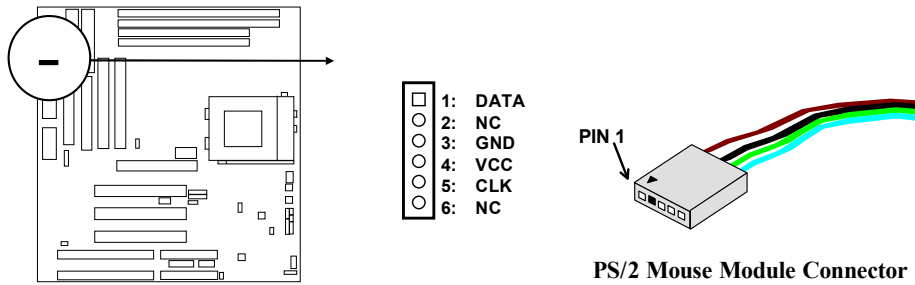
PS/2 Mouse Module Connector
